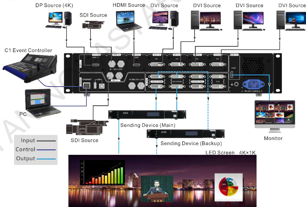
Figure 3-2 Connections for Switcher mode
