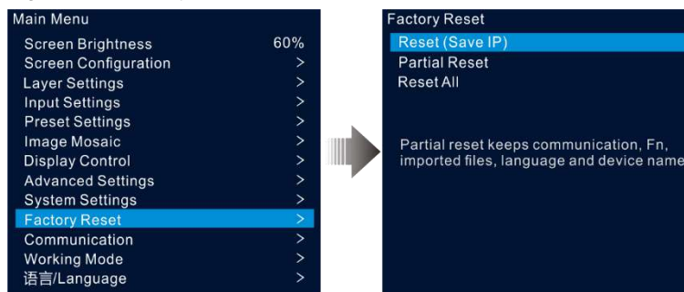
Figure 5-46 Factory reset
