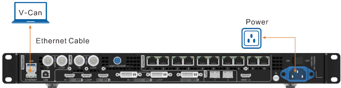
Figure 6-1 Hardware connection
